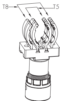
1. Mounting on linear tubes
